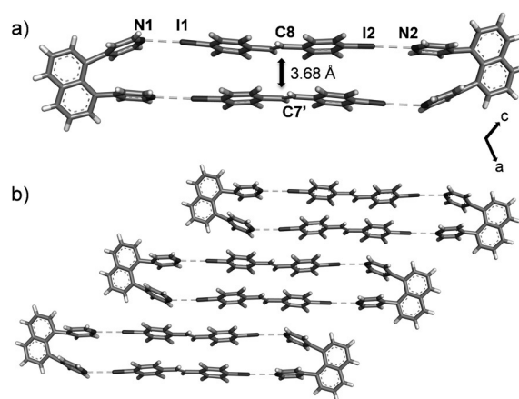
Figure 3. The X-ray crystal structure of 2( DPN ):2( 1 ), showing a) the halogen bonds facilitating the formation of the four-component 0D assembly and b) extended packing. The highest occupancy of DPN is shown.
